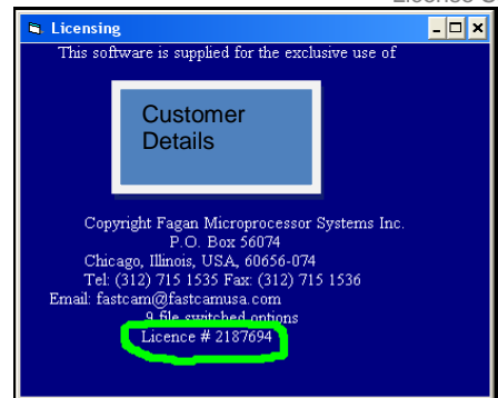
License Screen
